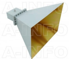
LB-975-15-C-7/16F Standard Gain Horn Antenna 0.75-1.12GHz 15dB Gain 7/16(DIN) Female
