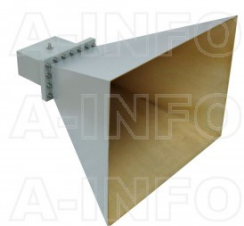
LB-975-15-C-NF Standard Gain Horn Antenna 0.75-1.12GHz 15dB Gain N Type Female
